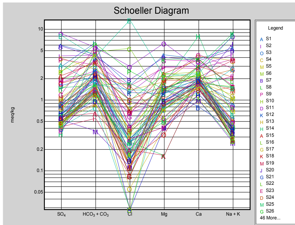
Figure 4: Schoeller Plot for groundwater parameters in the study area.
