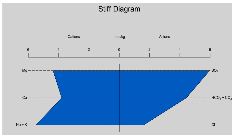
Figure 5: Stiff Plot for groundwater parameters in the study area.
