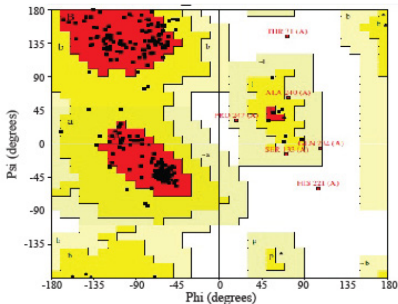
Plot statistics
